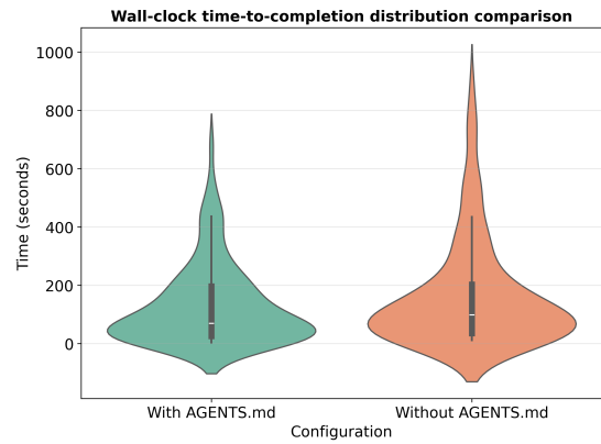
Figure 1: Wall-clock time-to-completion distributions for agent runs with and without AGENTS.md
